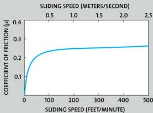
FIGURE 6: COEFFICIENT OF FRICTION VS. SPEED
